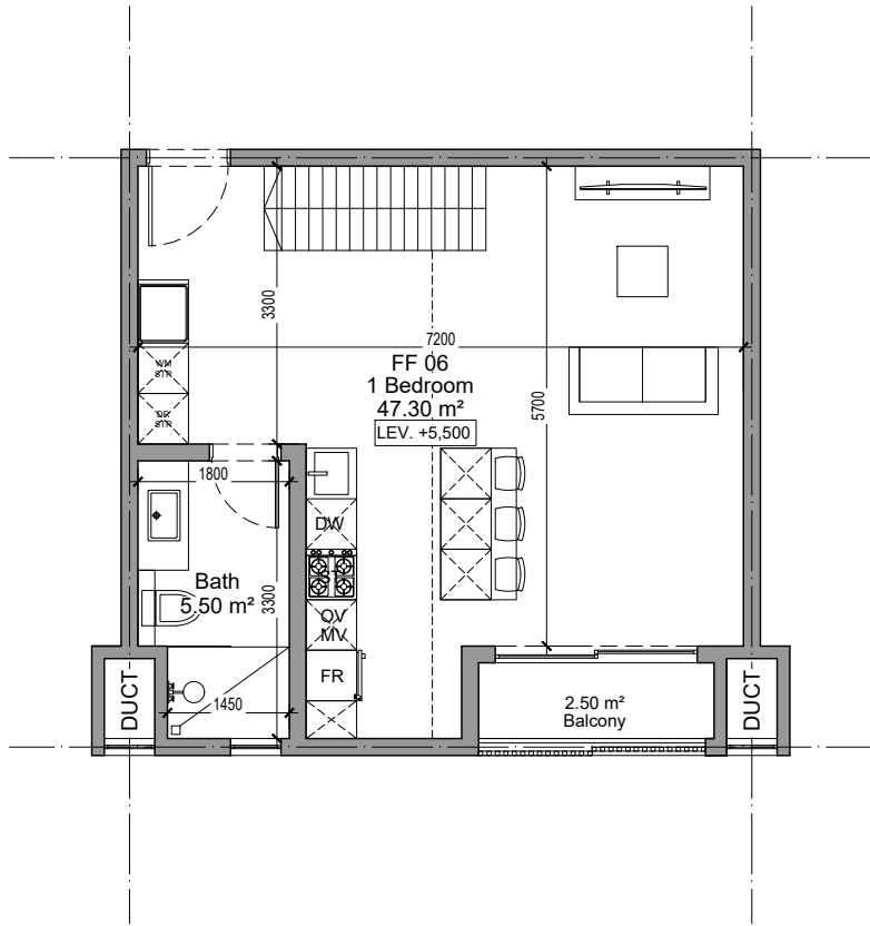
FIRST FLOOR [APARTMENT 6]
